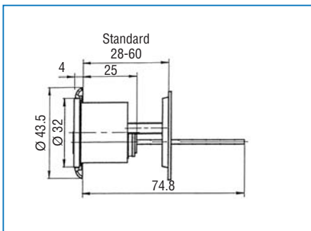
Rim cylinder 4509
