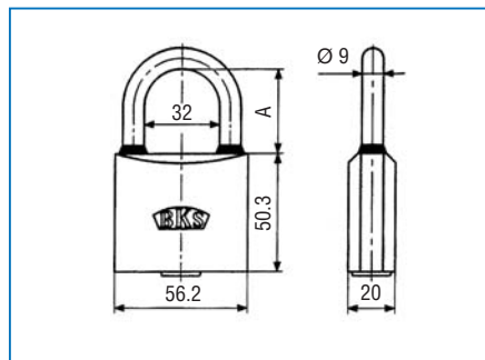
Brass padlock 4528
