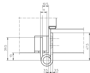
block frame
