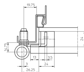
with blind rivet nut
