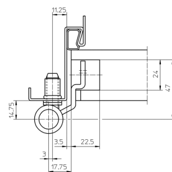
with blind rivet nut
